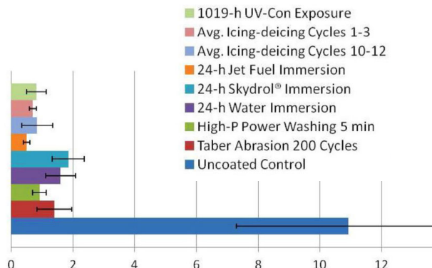
Figure 5: Ice Adhesion Strength (psi)
